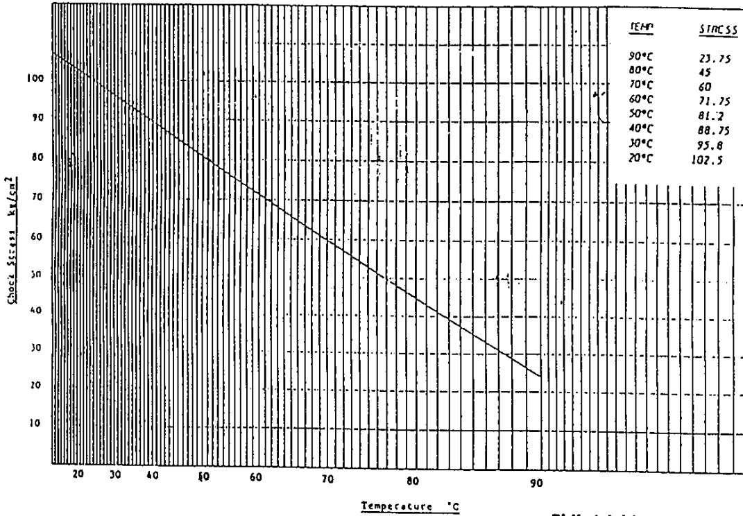
Permitted CHOCKFAST ORANGE® chock stress
